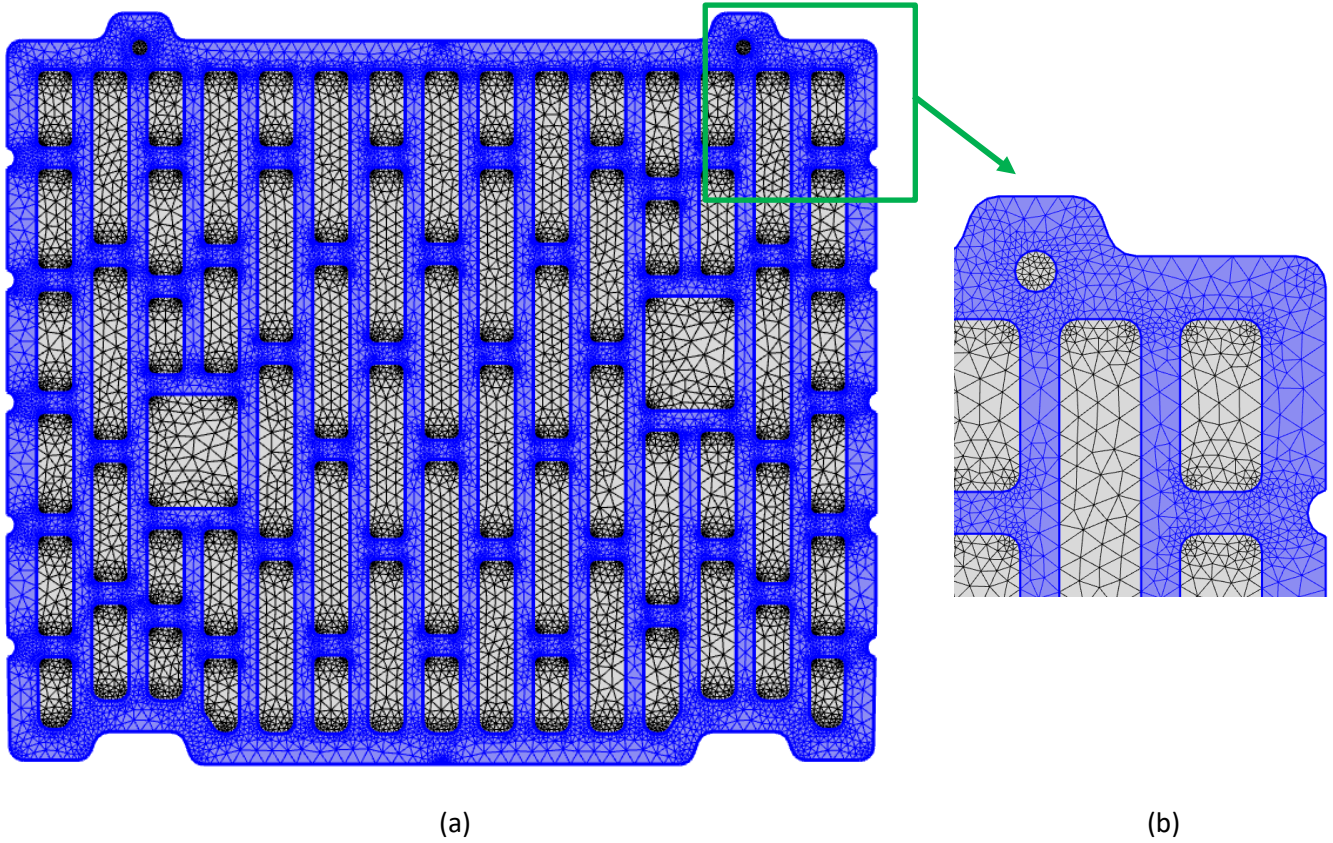
Fig.2. Schematic of the computational grid used (a) in the thermoblock (b) around the air hole.
